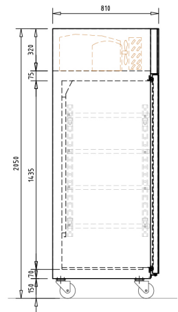
Section view
